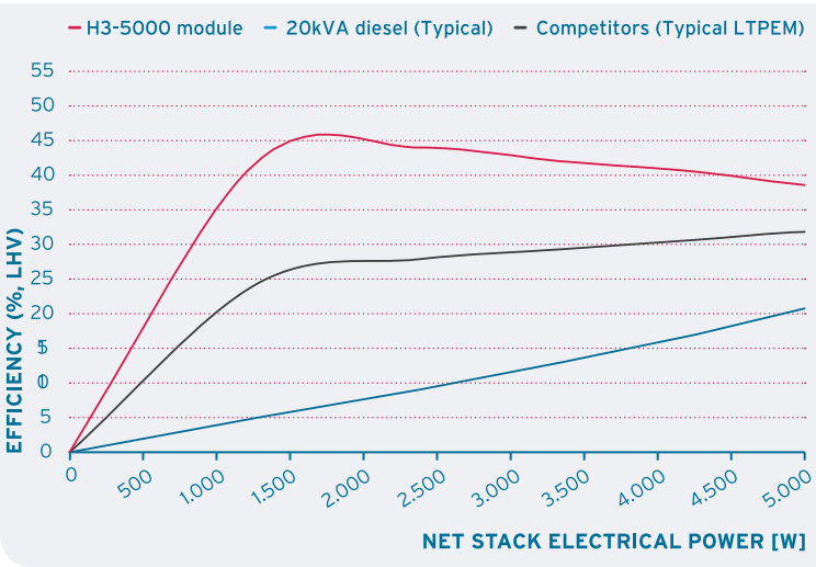
Typical level of efficiency of the Serenergy fuel cell and competing products
